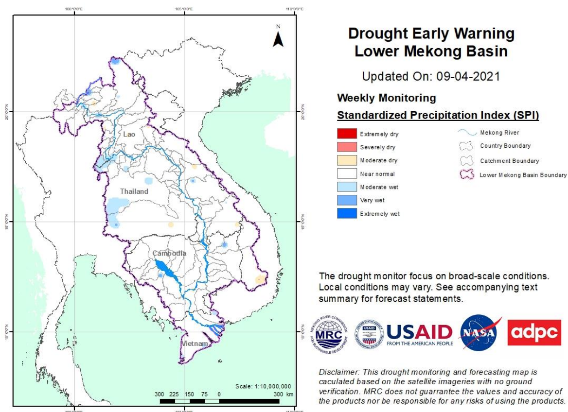
Figure 12: Weekly standardized precipitation index from 03 to 09 Apr 2021.
