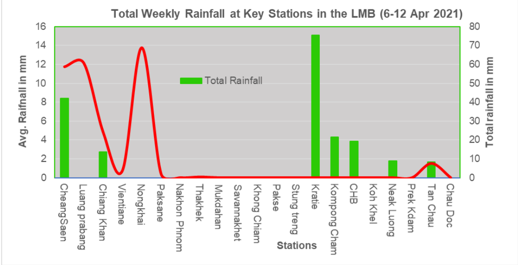
Figure 4: Weekly total rainfall at key stations in the LMB during 6-12 April 2021.
