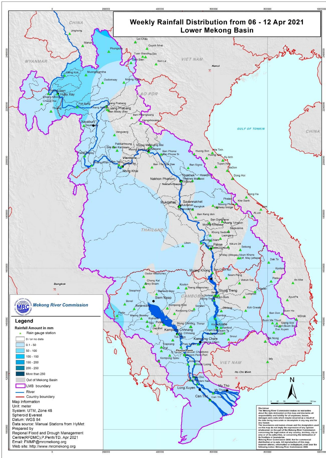
Figure 5: Weekly rainfall distribution over the LMB during 6 – 12 Apr 2021.
