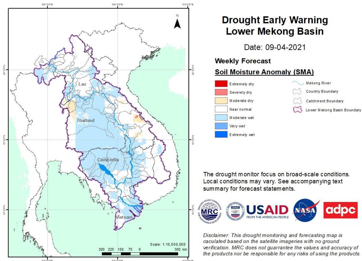
Figure 13: Weekly Soil Moisture Anomaly from 03 to 09 Apr 2021.
