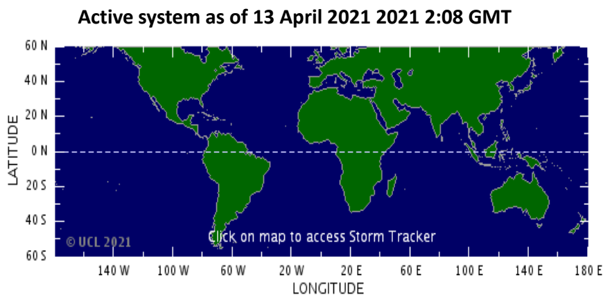
Figure 3: A Tropical Depression risk observed on 13 April 2021.
