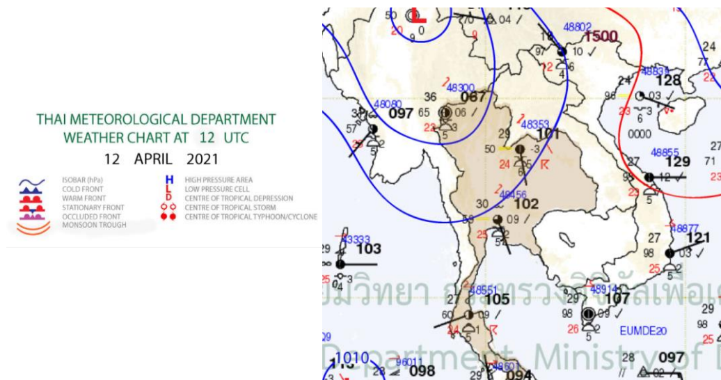
Figure 1: Summary of weather conditions over the LMB.
